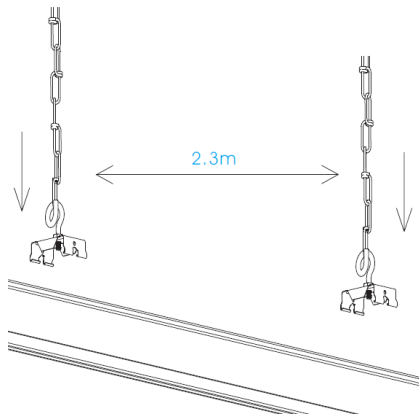
Installation distances
