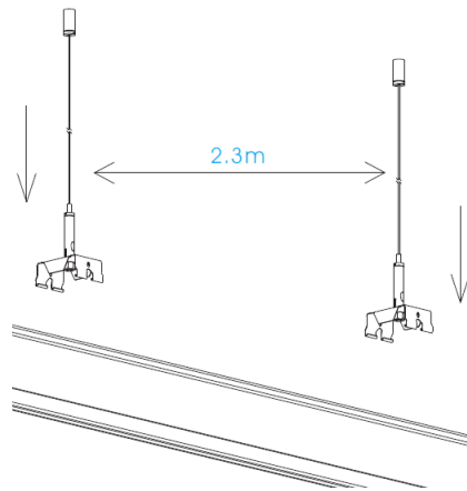
Steel cable
